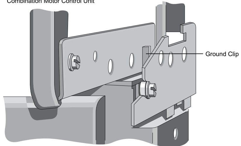
Combination Motor Control Unit
