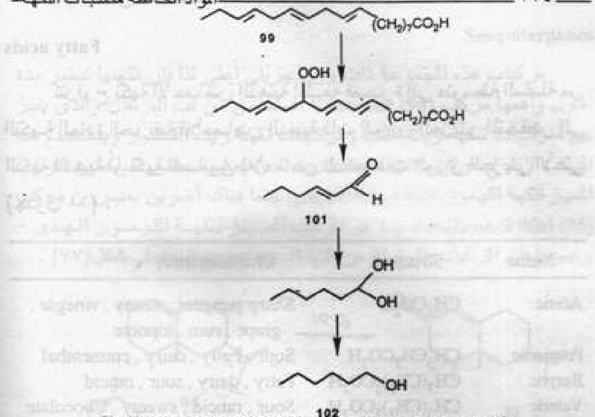
شكل (٧٩) Unsaturated fatty acid precursor to green notes.
