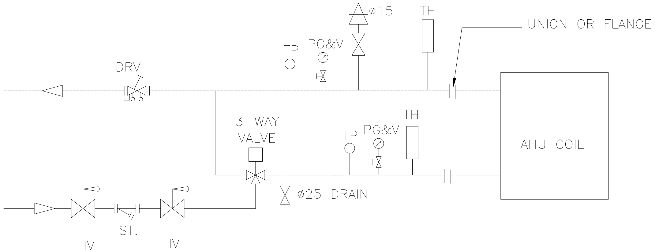
AHU PIPING CONNECTION DETAIL:
