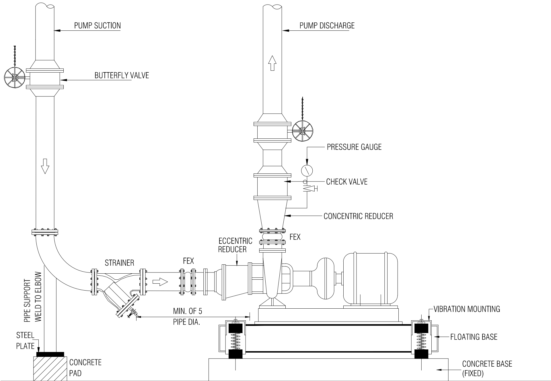
END SUCTION PUMP DETAILS
