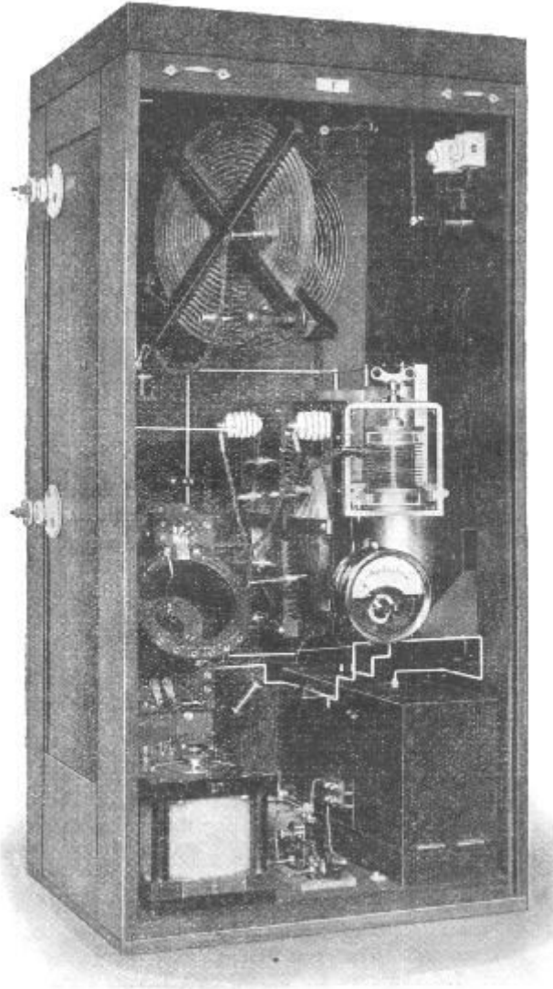
Fig. 2.- CABINET TYPE, WIRELESS INSTALLATION.
