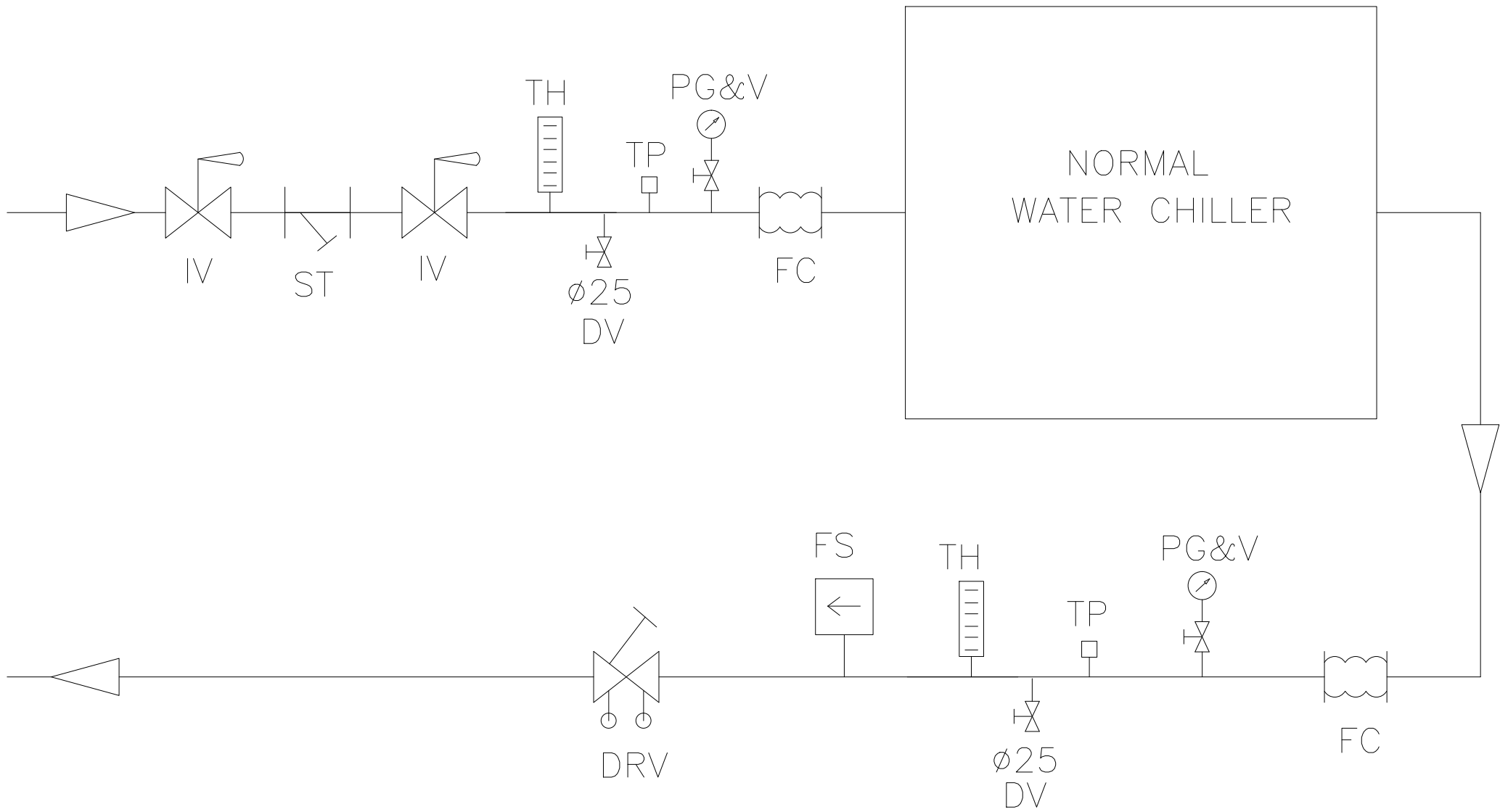
NORMAL CHILLER PIPING CONNECTION DETAIL:
