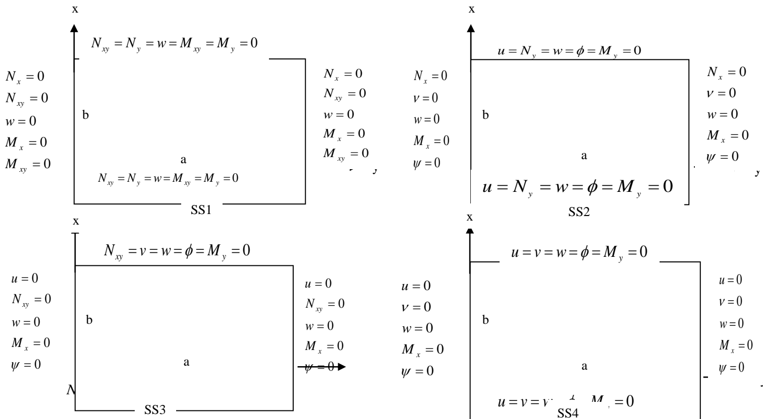
Fig. (1) Simply supported boundary conditions
