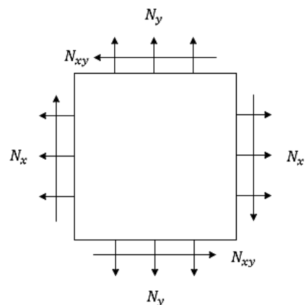
Fig. 4 External forces acting on an element
