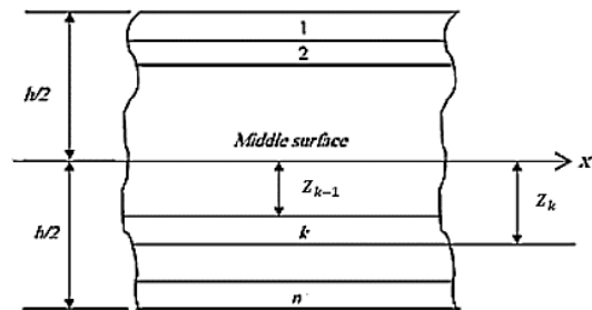
Fig. 3 Geometry of an n-layered laminate
