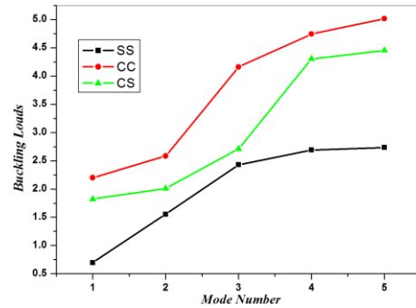
Fig. 6 Effect of boundary conditions
