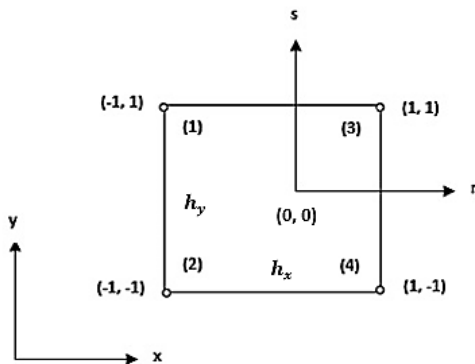
Fig. 5 A four noded element with local and global co – ordinates
