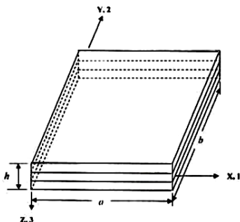
Fig. 1 The geometry of a laminated composite plate
