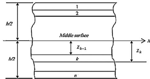
Fig. 3 Geometry of an n-layered laminate
