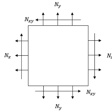
Fig. 4 External forces acting on an element
