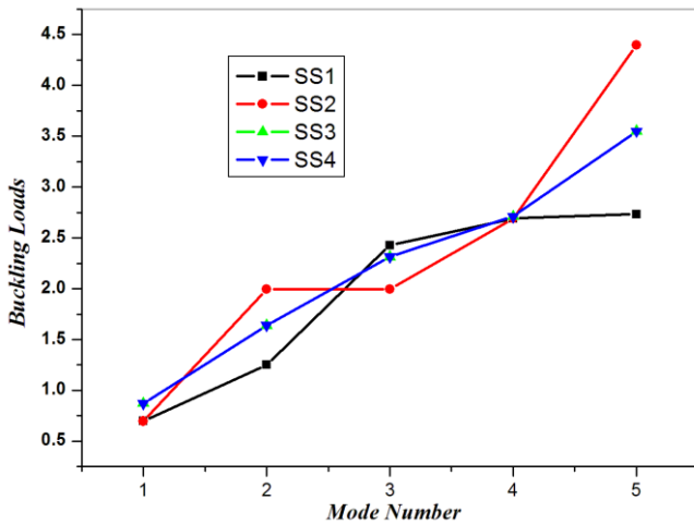
Fig. 6 Effect of lamination scheme for simply supported laminates
