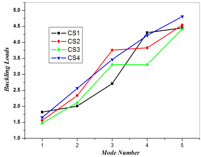
Fig. 8 Effect of lamination scheme for clamped – simply supported laminates
