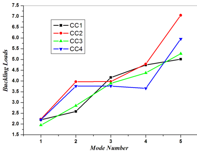
Fig. 7 Effect of lamination scheme for clamped – clamped laminates
