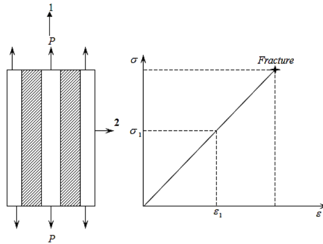
Fig. 4 Unidirectional lamina loaded in the fiber-direction
