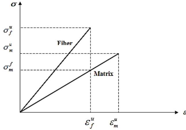
Fig. 2 Stress-strain relationships for fiber and matrix
