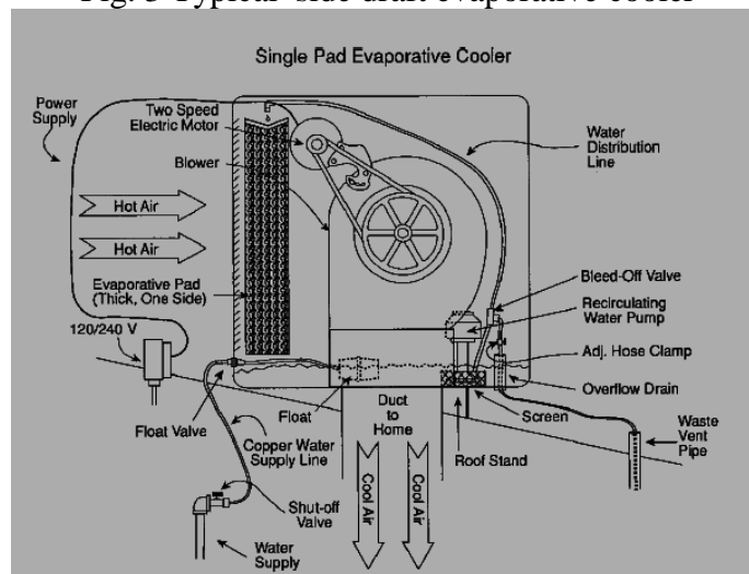
Fig. 4 Single pad evaporative cooler
