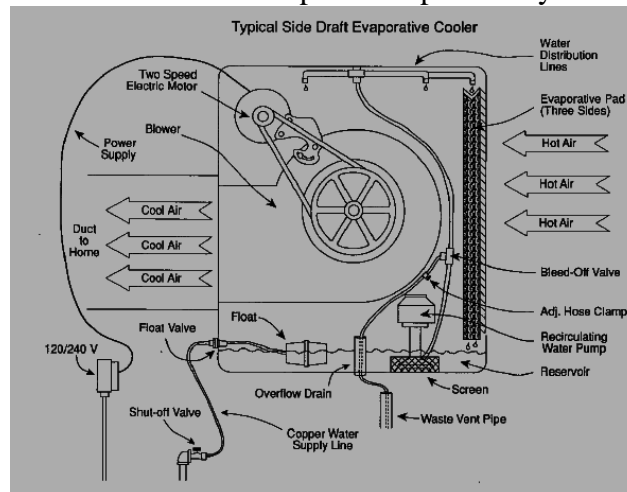
Fig. 3 Typical side draft evaporative cooler
